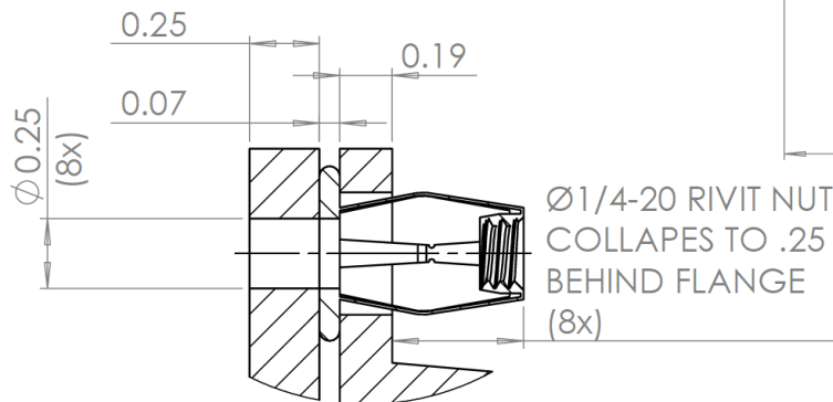
DETAIL B
